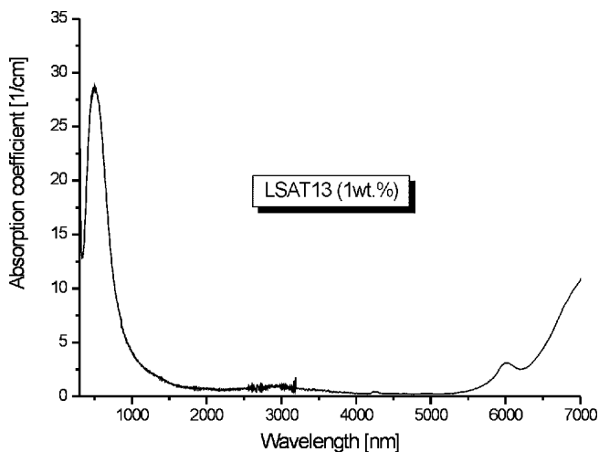
Fig. 2. Room temperature absorption coefficient of LSAT:Ti (LSAT13) single crystal in the range 200–7000 nm.
