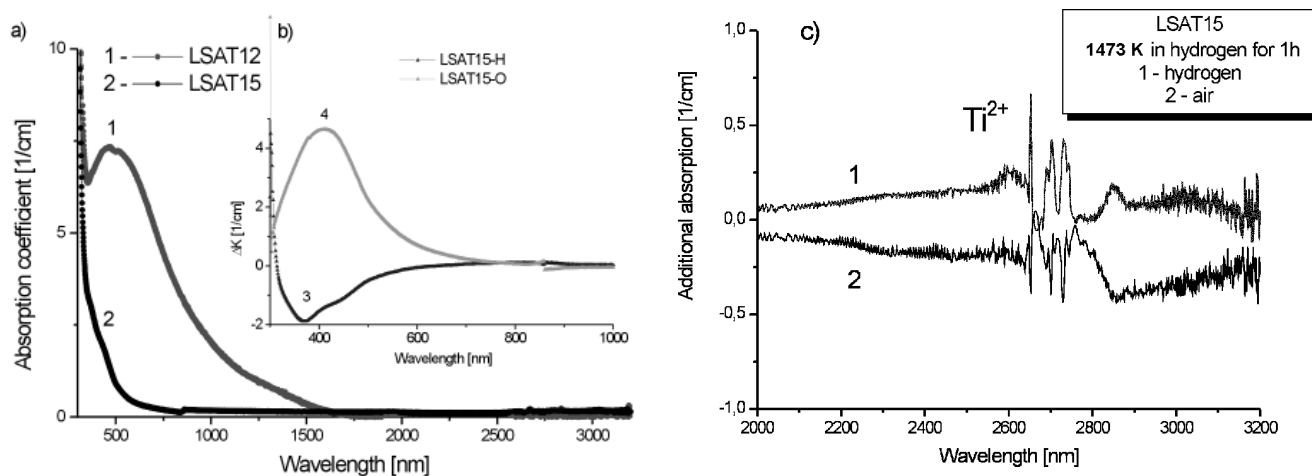
Fig. 5. a) – Room-temperature absorption coefficient of LSAT12 (1) and LSAT15 (2) samples in the range 300–3200 nm; b) – additional absorption of LSAT15 sample after annealing in hydrogen at 1473 K (3) and in air at 1673 K (4); c) – the same picture as b) in the range 2000–3200 nm.
