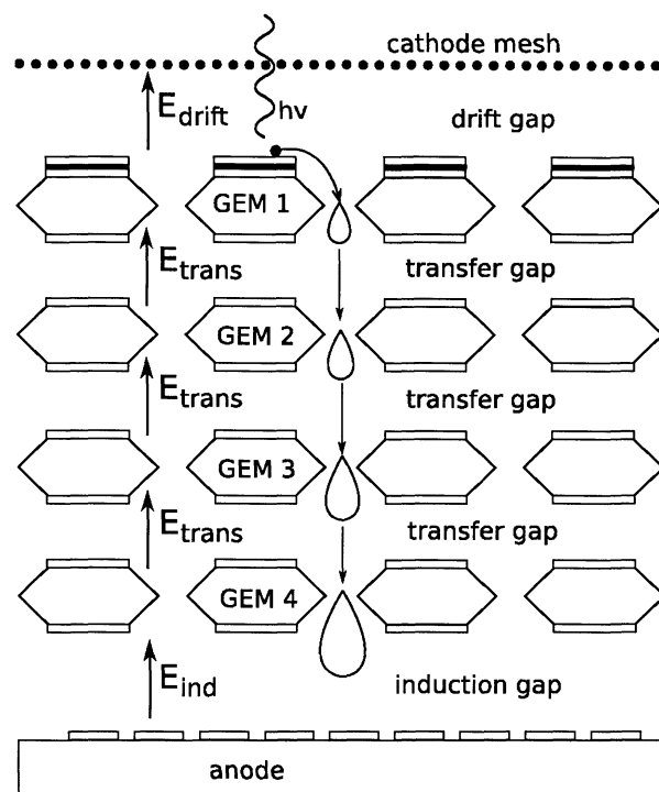
Fig. 3. Schematic drawing of multistage GEM set-up.
