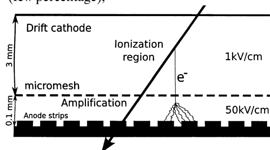
Fig. 4. Schematic drawing of MICROMEGAS detector.
