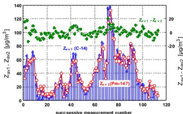
Fig. 4. Particulate matter concentration Z_{av} measured with two separate instruments fitted with PM10 samplers and two different beta-ray sources: C-14 and Pm-147 (1–14 March 2008, to the north of Warsaw).
