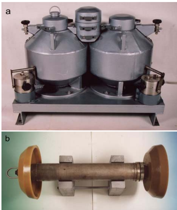
Fig. 5. Leakages testing at oil pipelines. a – methyl bromide generator ( \text{Br-82} ); b – “Pig” with gamma radioactivity measuring probe and recording system inside [7].
