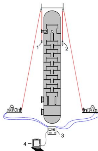
Fig. 6. Scheme of distillation column gamma scanning system [9]. 1 – gamma source with collimator; 2 – detector; 3 – radiometer; 4 – PC.
