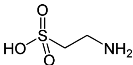
Fig. 1. Molecular structure of taurine.
