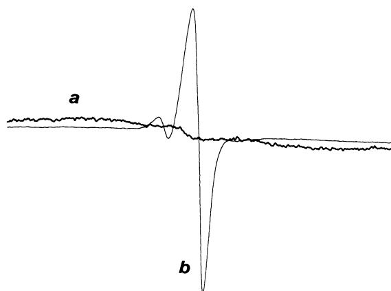
Fig. 2. (a) EPR spectrum of non-irradiated EVAPT20 rods, (b) EPR spectrum of EVAPT20 rods irradiated to 3 kGy.
