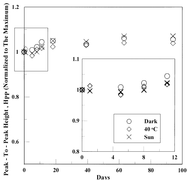
Fig. 5. Peak-to-peak heights ( H_{PP} ) of S_1 as a function of post-irradiation time (days) in different conditions over 94 days after irradiation, the inset clarifies the data of the first 11 days.
