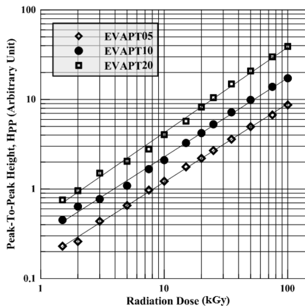
Fig. 4. Dose response curves of the EVAPT05, EVAPT10, and EVAPT20 rods at different doses from 1.5 to 100 kGy.
