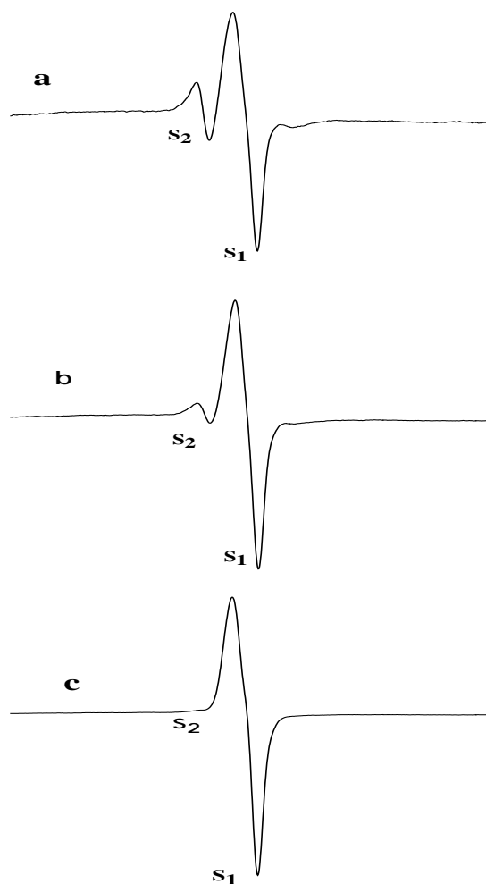
Fig. 3. EPR spectra of irradiated taurine samples (EVAPT20). EPR spectrum at 1.5 kGy (a), 3 kGy (b), and 50 kGy (c).
