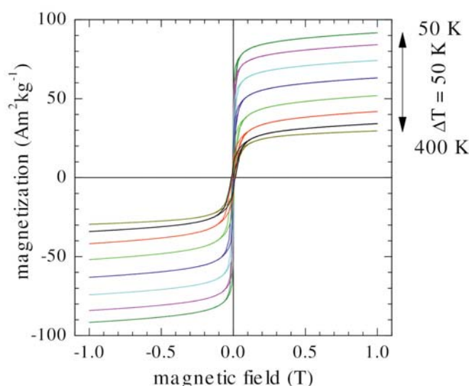
Fig. 4. Hysteresis loops measured at temperatures from 50 K to 400 K ( \Delta T = 50 K) upon as-quenched ^{57}\text{Fe}_{81}\text{Mo}_9\text{Cu}_1\text{B}_9 alloy.
