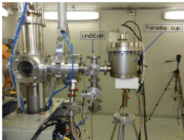
Fig. 7. Faraday cup installed on the BTL.
