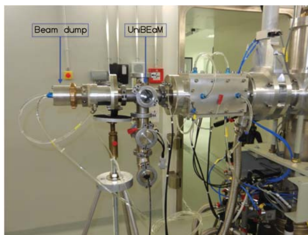
Fig. 4. The UniBEaM detector installed on the BTL in the Bern cyclotron laboratory.
